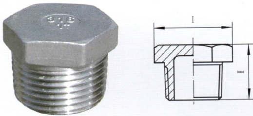
HEX PLUG
