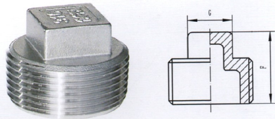
SQUARE PLUG
