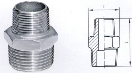
REDUCED HEX NIPPLE
