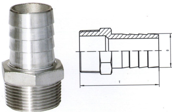
HOSE NIPPLE (HON)
