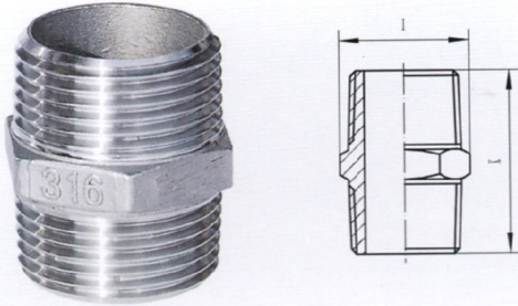
HEX NIPPLE
