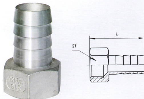
HOSE NIPPLE (HON-F)
